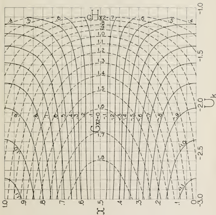
Chart 18— G_x and CH_x in attenuating band; \nu_1 neglected.
