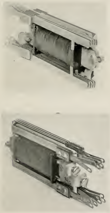
Fig. 13—"E" type relay
