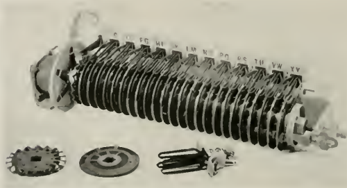
Fig. 21—24 cam sequence switch
