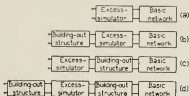
Fig. 11—Abstract Diagrams of Complete Networks for Simulating Characteristic Impedance of Loaded Line
