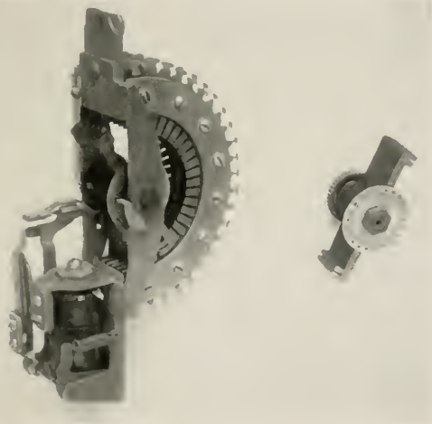
Fig. 23—Step-by-step rotary switch
