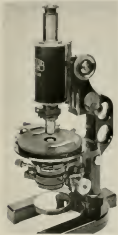
Fig. 2—Research type of microscope by Zeiss. Large barrel for photo-micrography; revolving mechanical stage, and sliding objective changers.
