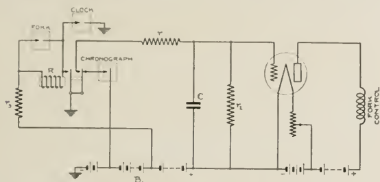
Fig. 2—Clock Control of Fork Frequency. (Schematic Diagram)
