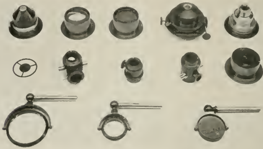
Fig. 7—Condensers and illuminators used in microscopy
