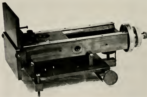
Fig. 4—Photograph of the Boltzmann Interferometer. ( Physical Review )
