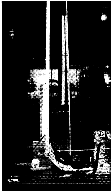
Figure 1.—Photograph of the inside of the vacuum chamber showing the two vertical aluminum plate electrodes and a painting hanging on the ground plate (to the right).
