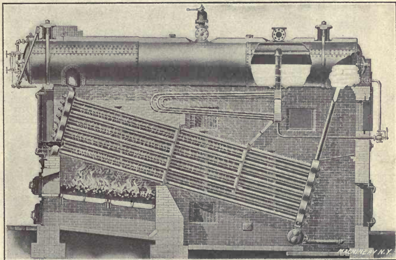
Fig. 10. Babcock and Wilcox Water-tube Boiler
