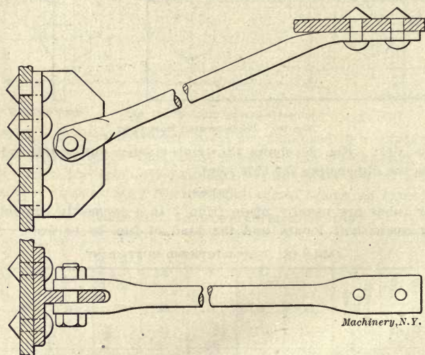
Fig. 21. Diagonal Type Boiler Brace
